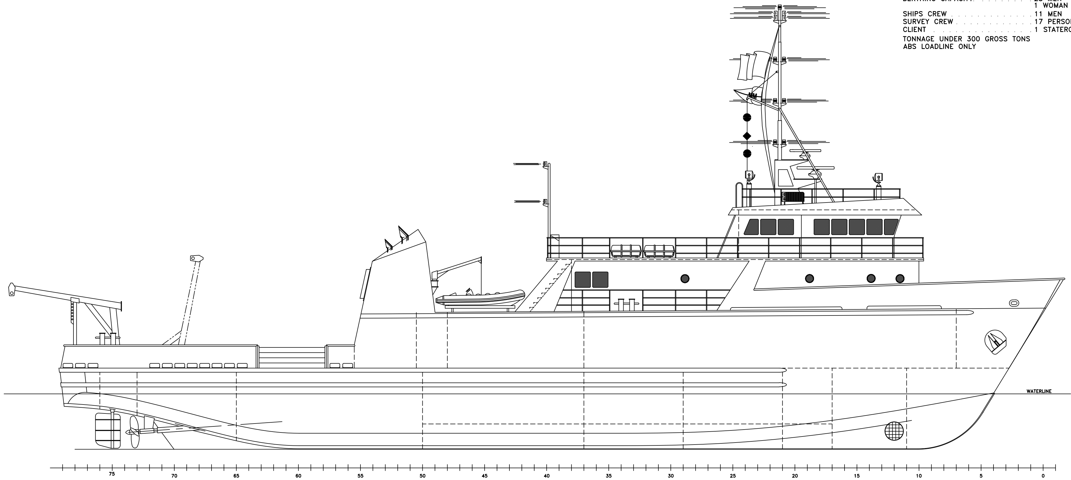
OUTBOARD PROFILE
