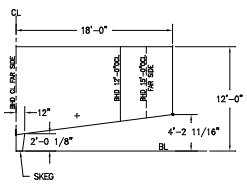
FRAME 53 LKG AFT
