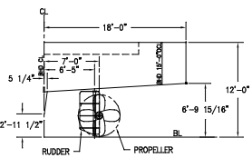
FRAME 65 LKG AFT
