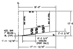
FRAME 24 LKG AFT
