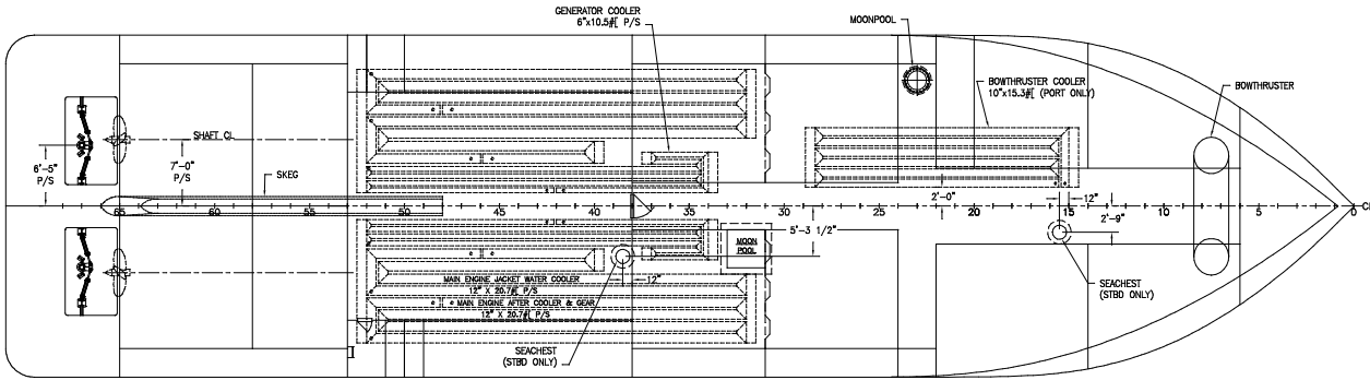
BOTTOM PLAN VIEW
