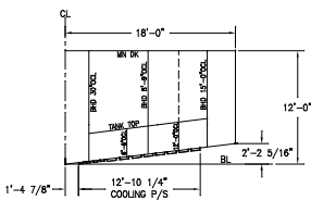
FRAME 38 LKG AFT
