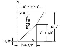
FRAME 6 LKG AFT
