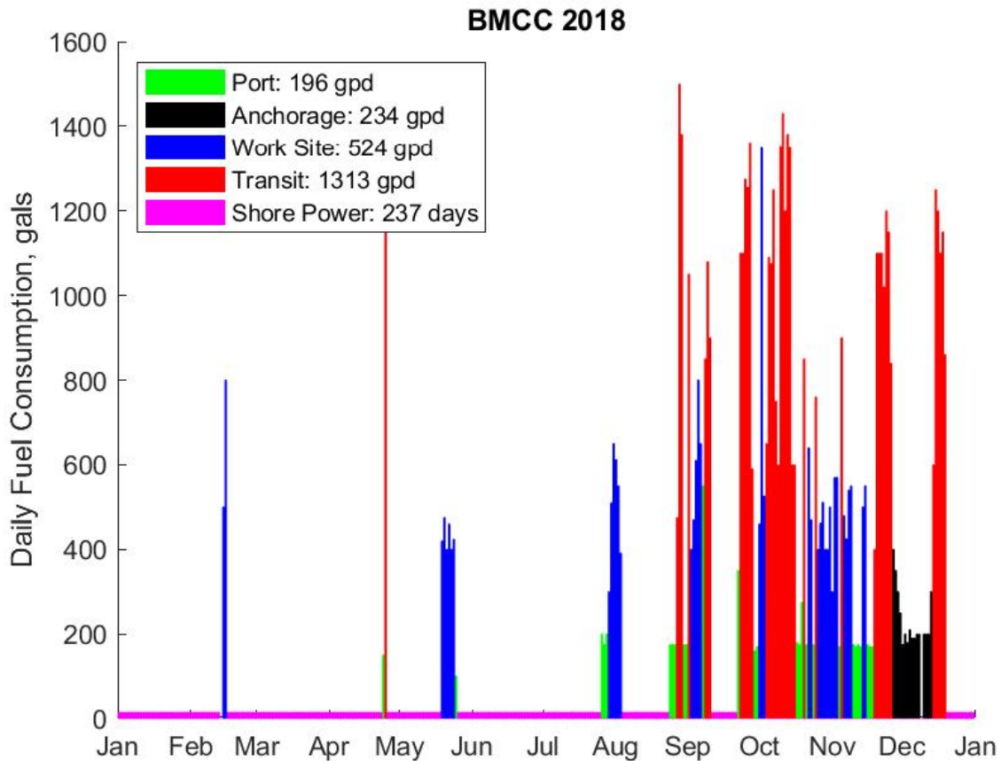
Figure 2 - Daily energy usage by category for the R/V Brooks McCall in 2018
