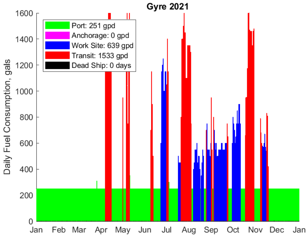
Figure 2 shows the vessel operations for 2021 for the R/V Gyre.
