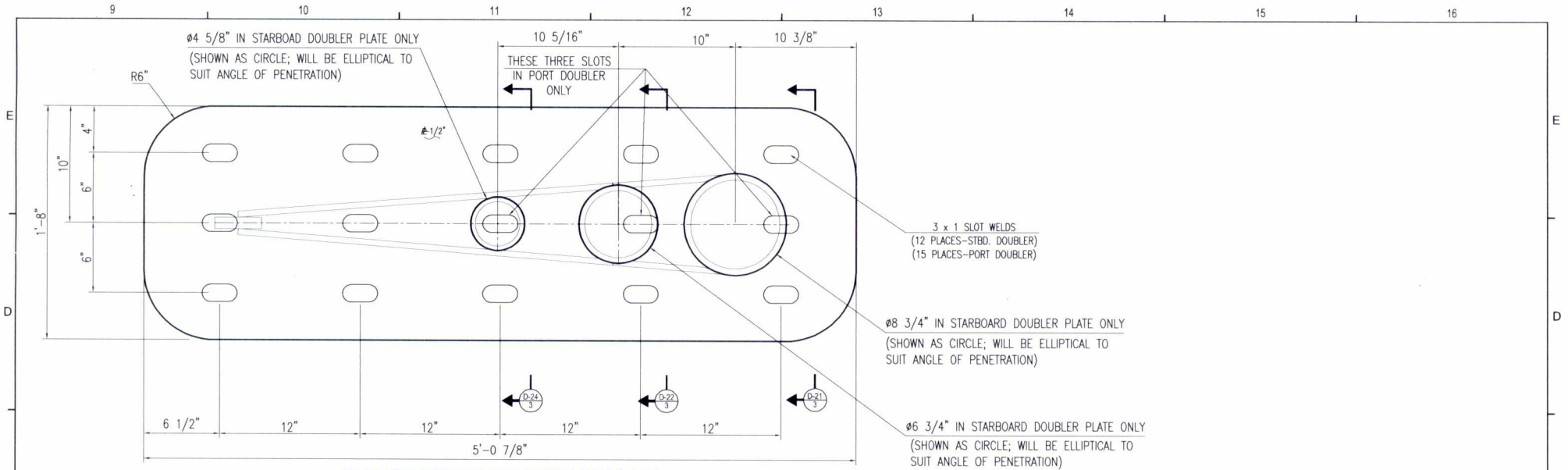
PLAN OF STARBOARD DOUBLOR PLATE PORT SIMILAR AS NOTED 3"= 1'-0"
