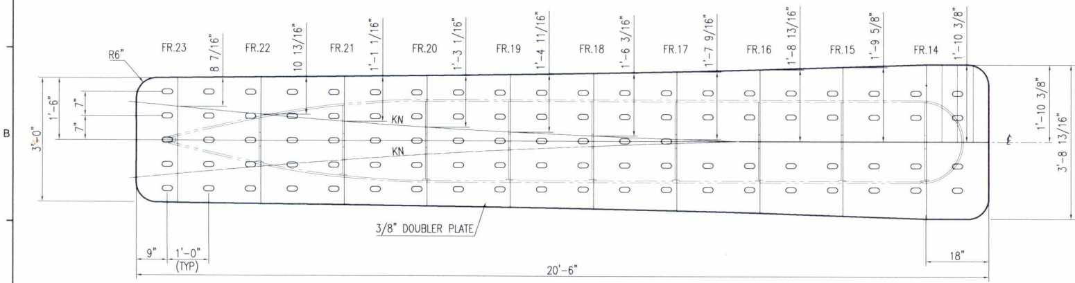
PLAN OF CENTERLINE DOUBLOR PLATE OFFSETS AT FRAMES SHOULD BE FIELD VERIFIED 1/12" = 1'-0"
