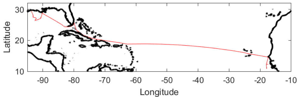
Figure 1 - Route taken by the R/V Gyre in 2018.
