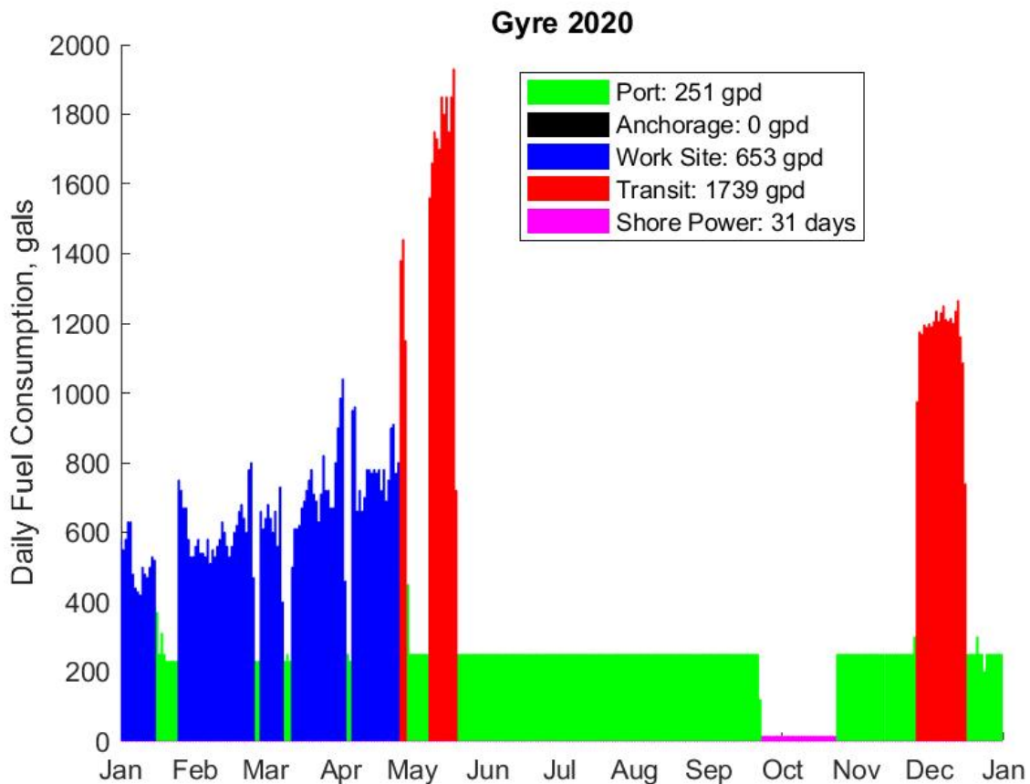
Figure 2 - Daily energy usage by category for the R/V Gyre .
