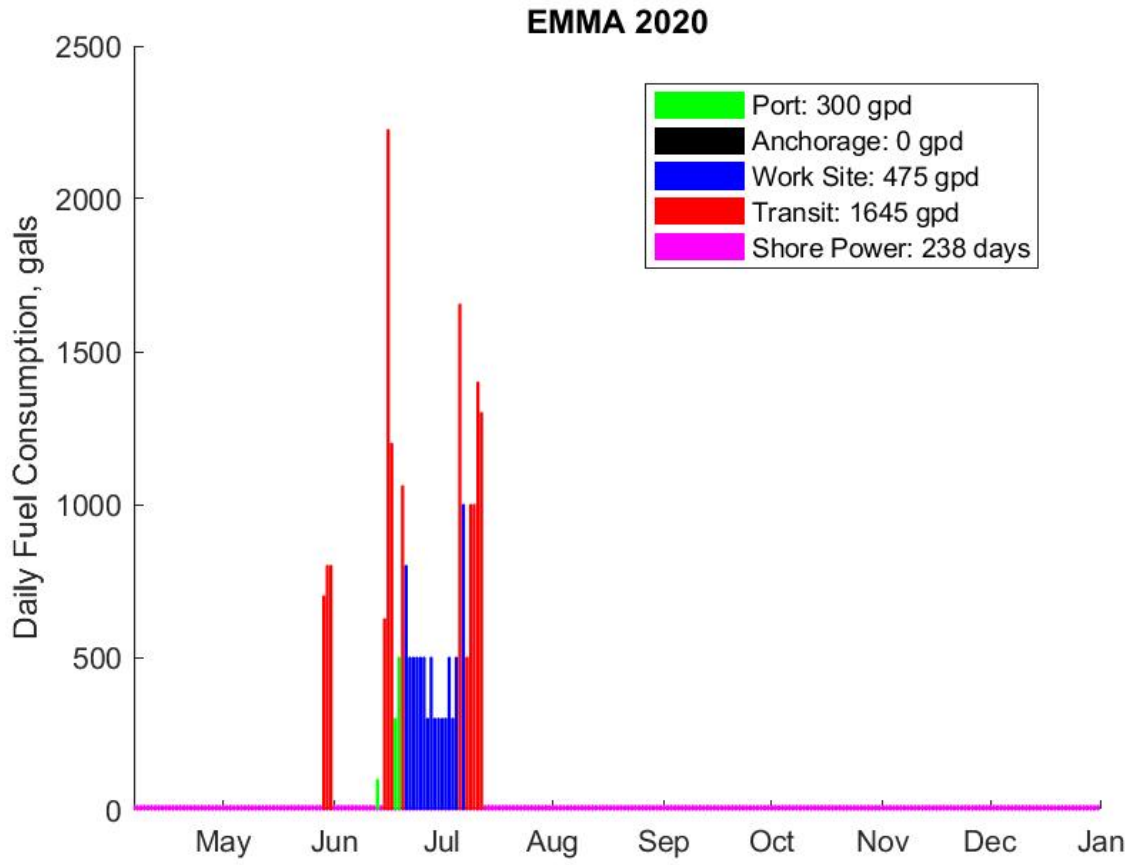
Figure 1 - Daily energy usage by category for the R/V Emma McCall in 2020
