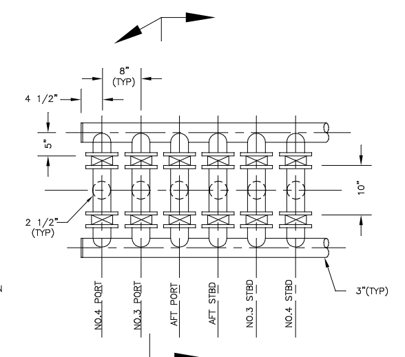
AFT BALLAST MANIFOLD SCALE: NONE
