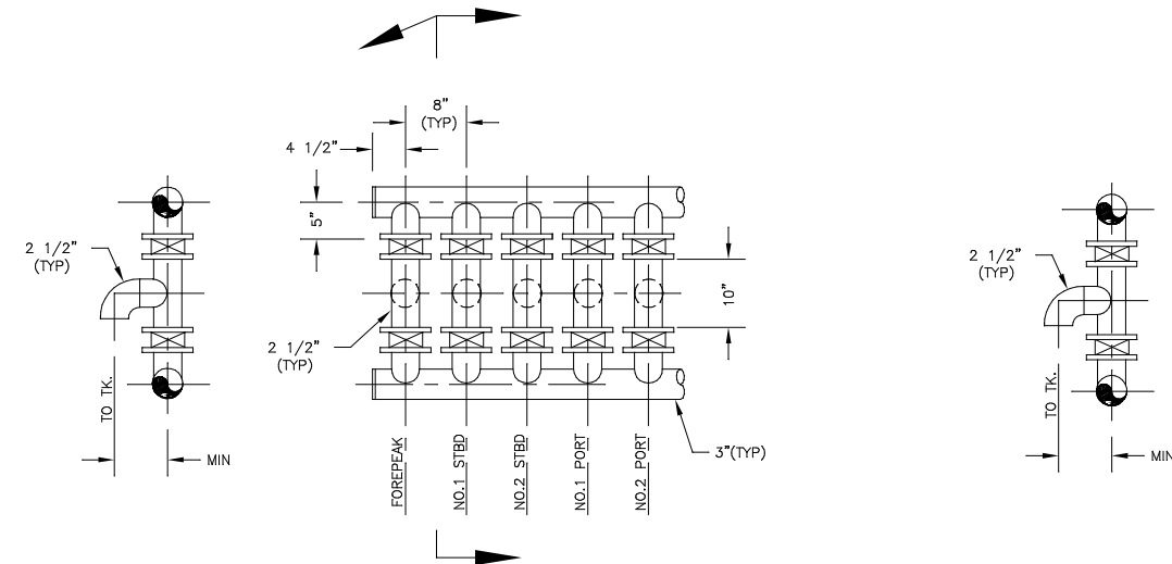
FWD BALLAST MANIFOLD SCALE: NONE
