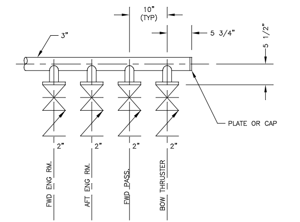
BILGE MANIFOLD DETAIL SCALE: NONE
