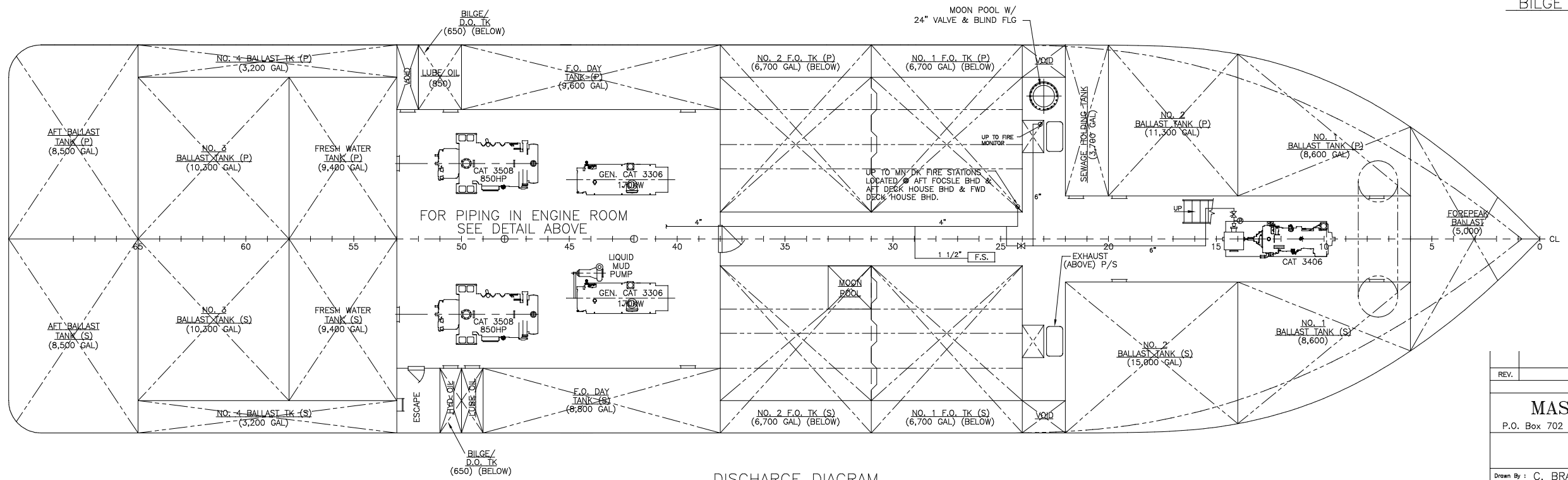
DISCHARGE DIAGRAM
