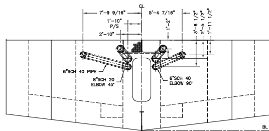
SECTION C-C FWD E.R. BHD - LKG FWD
