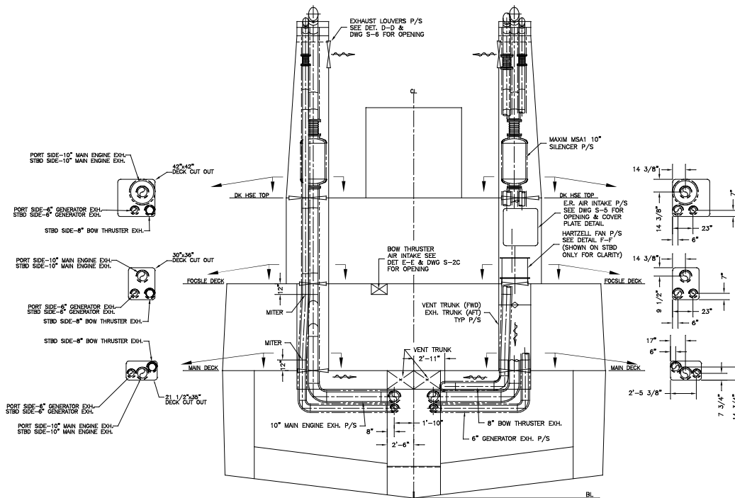
SECTION B-B LKG FWD
