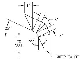
DETAIL H-H TYP. EXHAUST OUTLET SCALE: 1"=1'-0"
