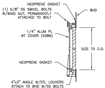
DETAIL E-E SCALE: NONE
