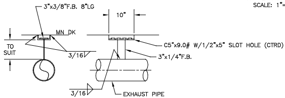
DETAIL G-G PIPE SLIDE SCALE: 1"=1'-0"
