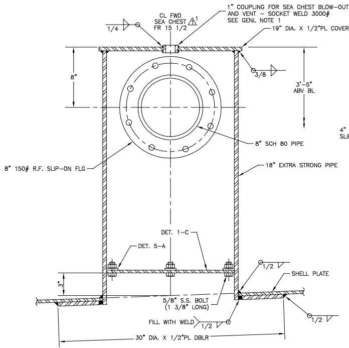
DETAIL 5-C FWD SEA CHEST - 2'-9" OFF CL (S) \Delta^1 SCALE: 3"=1'-0"
