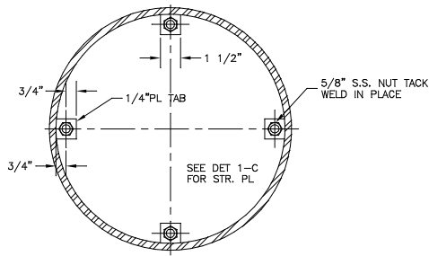
DETAIL 5-A BOLT LCTN FOR STRAINER PL SCALE: 3"=1'-0"
