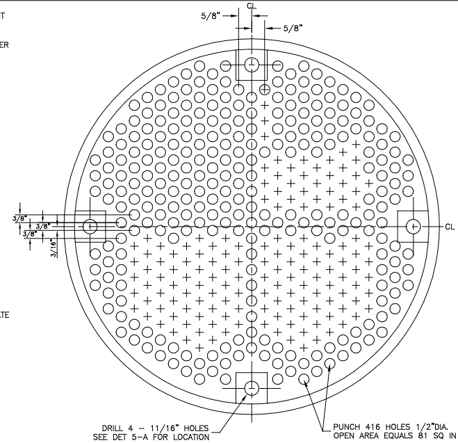
DETAIL 1-C STRAINER PLATE SCALE: HALF SIZE
