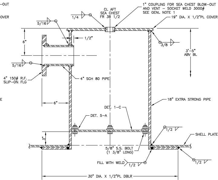
DETAIL 3-C AFT SEA CHEST - 5'-3 1/2" OFF CL (S) \Delta^1 SCALE: 3"=1'-0"
